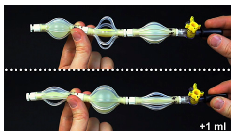
Fig. 6. Snapshots of a combined actuator with (L_{\text{braid}}, L_{\text{tube}}) = (40, 28) , (44, 30) , and (50, 24) mm. The numerical analysis predicts a (2, 1) state transition at v = 29 mL (see gray triangle in Fig. S7A–C). The combined actuator is inflated to v = 28 mL, and then decoupled from the syringe pump and connected to a small reservoir containing only 1 mL of water. An additional volume of 1 mL supplied to the system is enough to trigger a significant internal volume flow of \sim 20 mL that results in the deflation of two segments into one segment (Movie S6).
