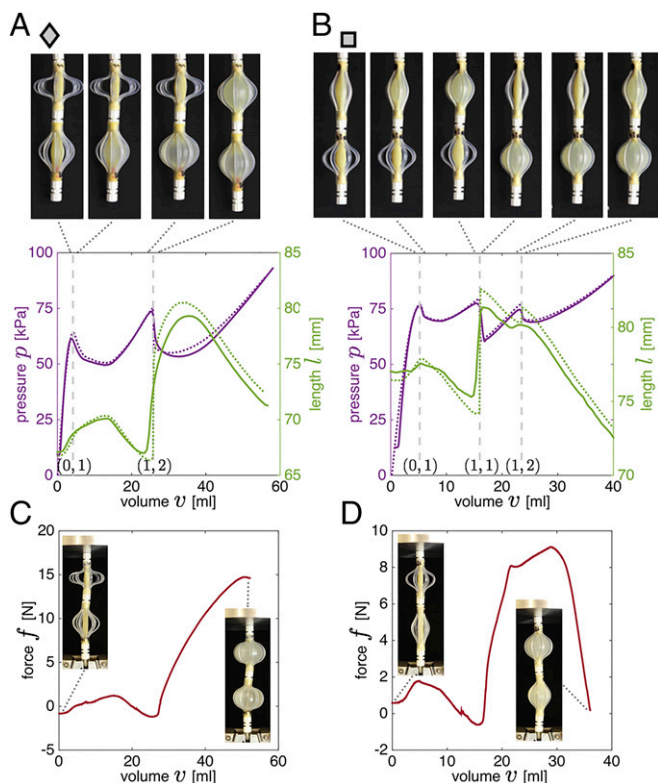
Fig. 5. (A and B) Experimental (solid lines) and numerical (dashed lines) pressure–volume curves for two soft actuators comprising n=2 fluidic segments. (A) Results for a combined actuator with (L_{\text{braid}}, L_{\text{tube}}) = (48, 30) and (50, 20) mm. The transitions for this actuator are highlighted by diamond markers in Fig. 4. Snapshots of the combined actuators 0.5 mL before and after each state transition (at v = 4, 26 mL) are also shown. (B) Results for a combined actuator with (L_{\text{braid}}, L_{\text{tube}}) = (44, 30) and (48, 26) mm. The transitions for this actuator are highlighted by square markers in Fig. 4. Snapshots of the combined actuators 0.5 mL before and after each state transition (at v = 5, 16, 24 mL) are also shown. Experimentally measured exerted force as a function of the supplied volume for a combined actuator with (C) (L_{\text{braid}}, L_{\text{tube}}) = (48, 30) and (50, 20) mm and (D) (L_{\text{braid}}, L_{\text{tube}}) = (44, 30) and (48, 26) mm with constrained ends.
